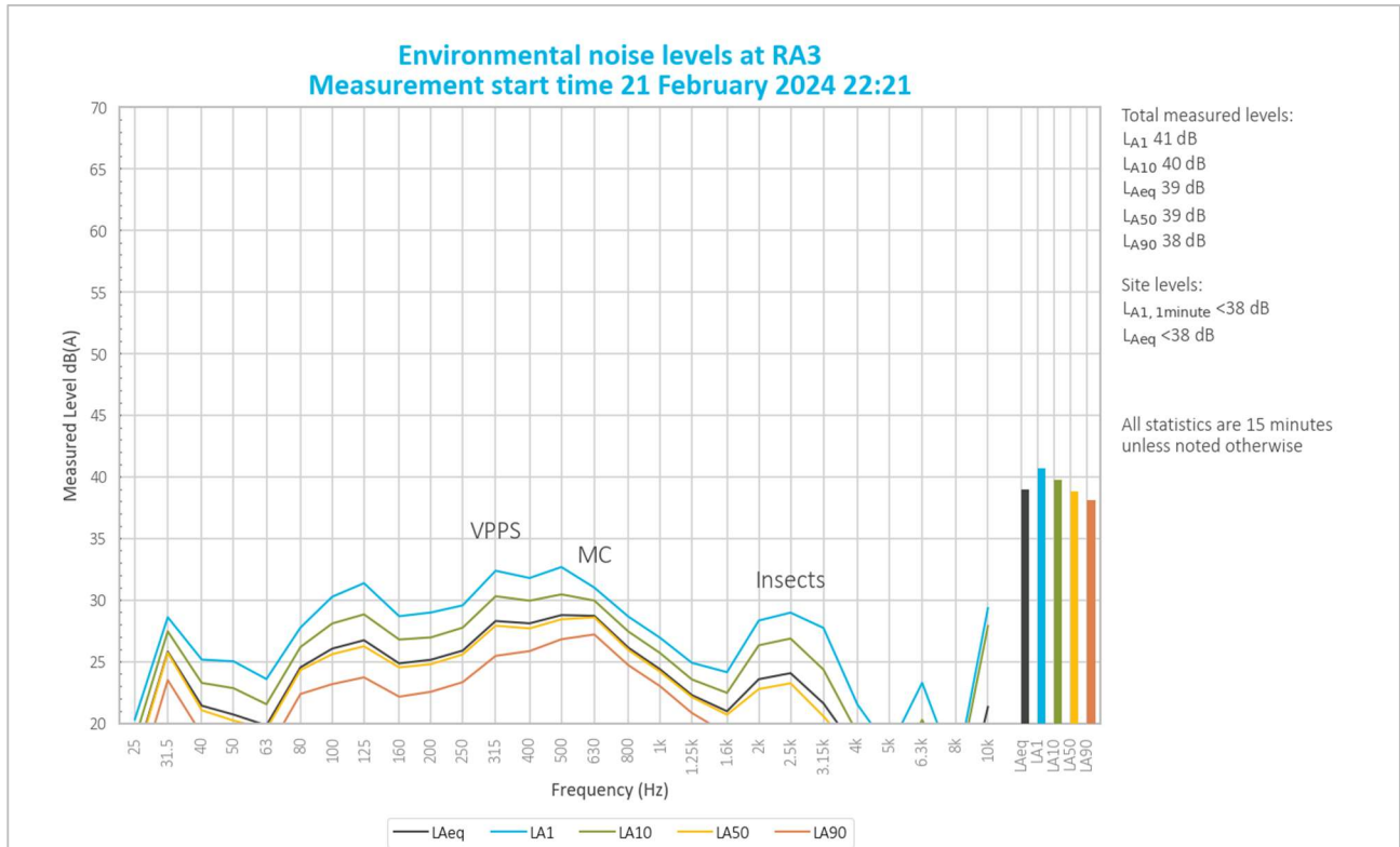
Figure 5.5 Environmental noise levels – RA3 (Kingfisher Shores) – Night
