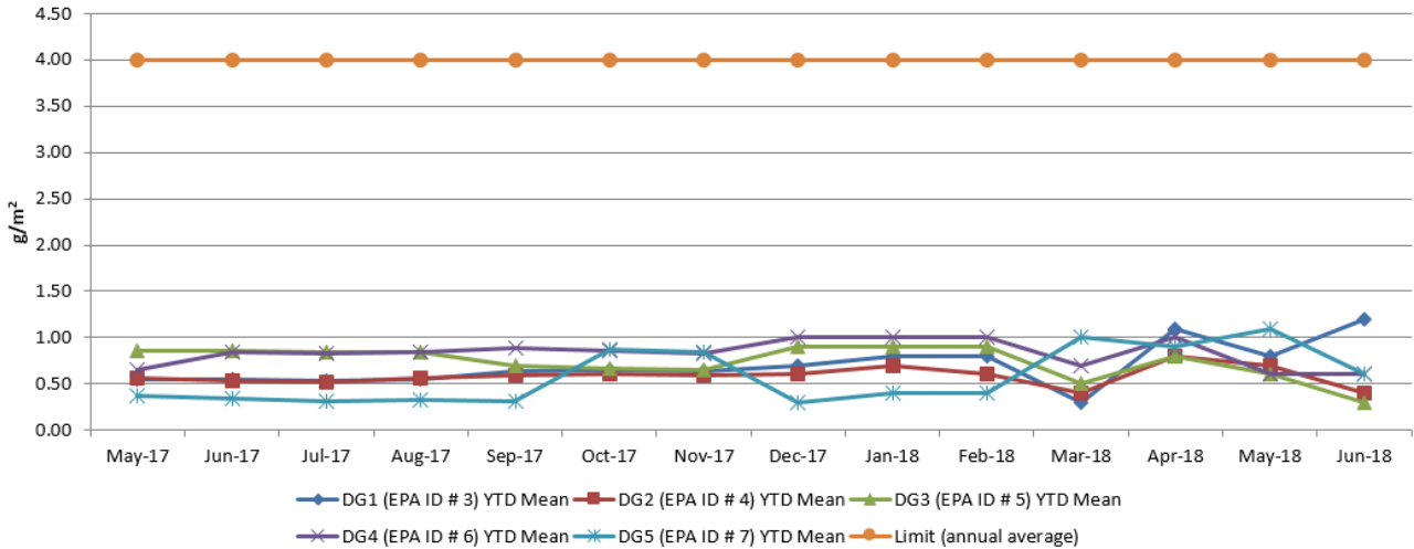
Yearly Rolling Average Depositional Dust Data
