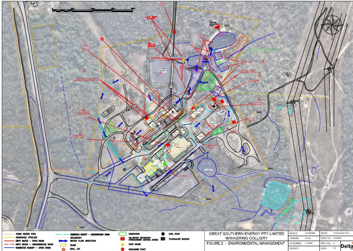
Figure 2 – Mannering Colliery Environmental Location Plan
